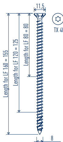
Locking screw: GoFix® S+ in stainless steel
